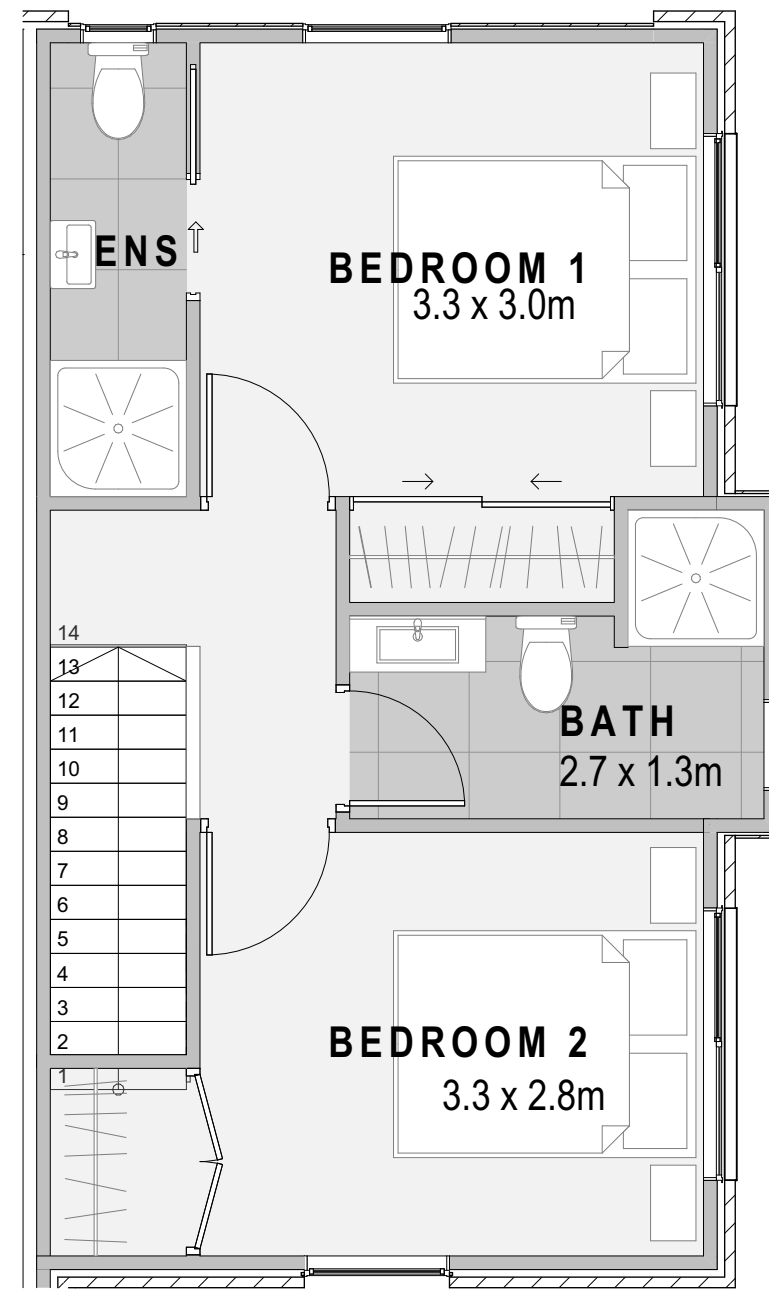
2 FIRST FLOOR PLAN 1:50
