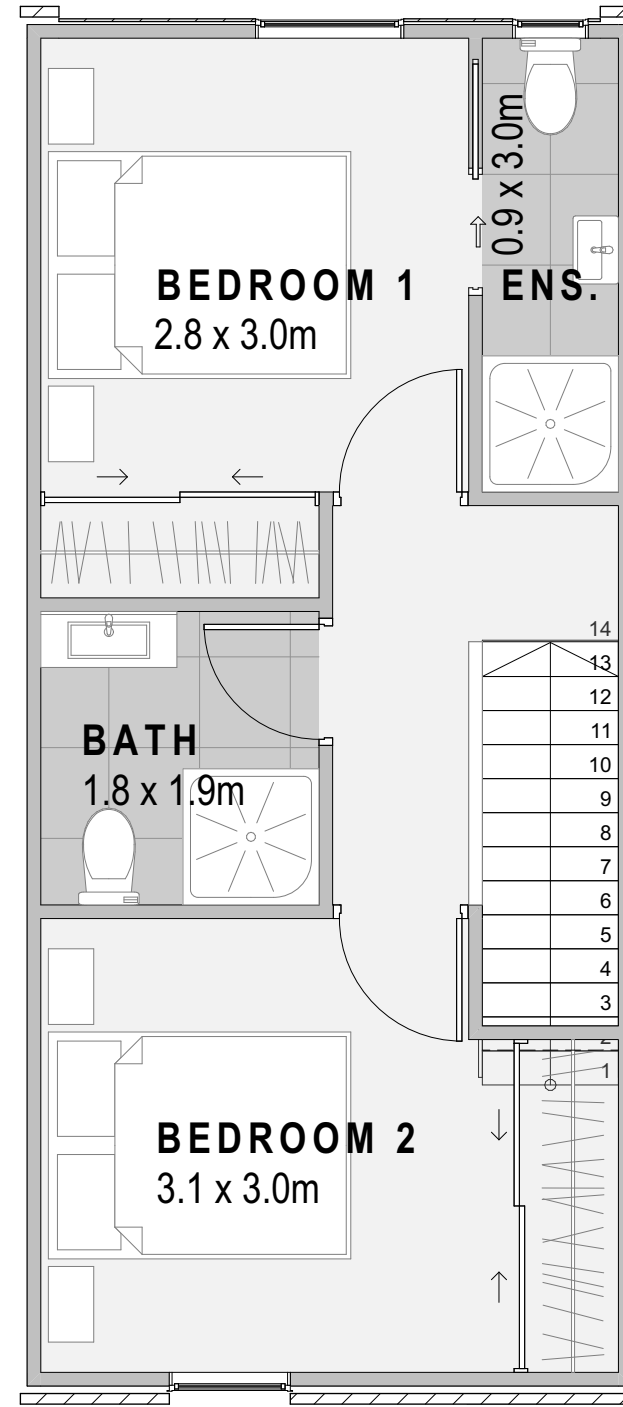
2 FIRST FLOOR PLAN 1:50
