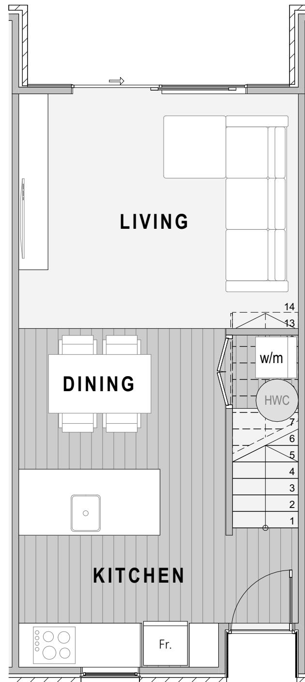
1 GROUND FLOOR PLAN 1:50
