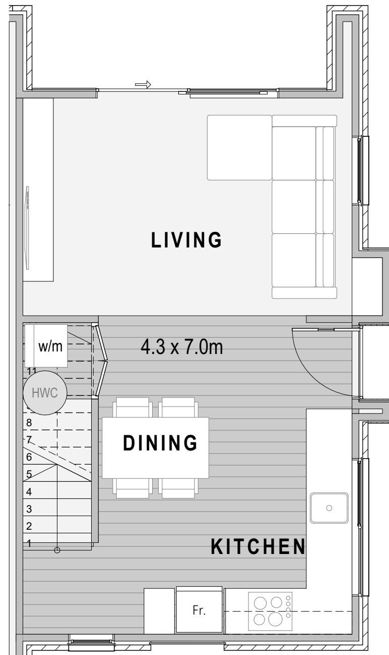
1 GROUND FLOOR PLAN 1:50
